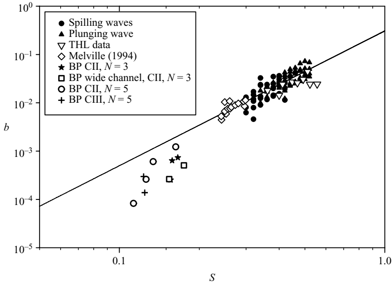
FIGURE 16. Plot of b versus S for SIO spilling and plunging waves along with the data of Melville (1994) and the THL data. Also shown are the data of Banner & Peirson (2007, BP). The solid line is a least-squares fit to the SIO data and has a slope of 2.77.
