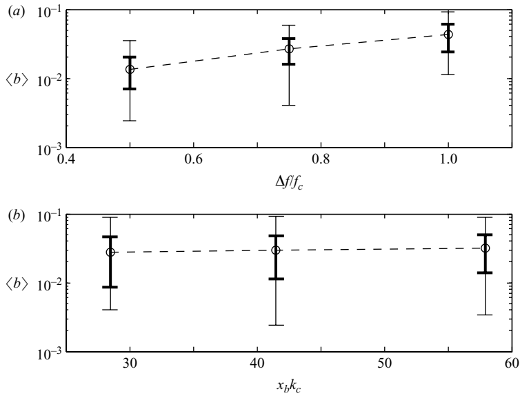
FIGURE 12. Plot of \langle b \rangle versus (a) \Delta f/f_c and (b) x_b k_c , where the average is over all samples for a given value of \Delta f/f_c or x_b k_c . The thin error bars span the maximum and minimum values within the average, and the thicker line is the standard deviation of the data.
