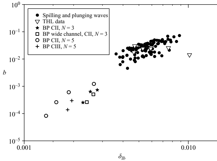
FIGURE 17. Plot of b versus \delta_{ib} for SIO spilling and plunging waves, along with THL data and that of Banner & Peirson (2007).
