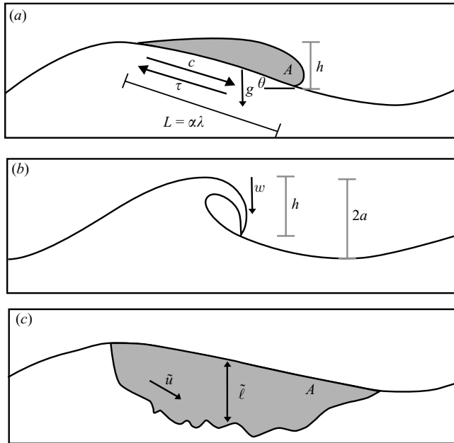
FIGURE 1. A definition sketch for (a) a spilling wave, (b) a plunging wave before breaking, and (c) a plunging wave after breaking. In (a) L is the length of the breaking region, \lambda the wavelength of the breaking wave, c the phase speed of the breaking wave, \tau the shear stress exerted by the breaking region on the underlying fluid, g acceleration due to gravity, \theta the angle of inclination, and A the area encompassed by the spilling wave. In (b) h is the height of the breaking region, 2a is the distance from the crest to the trough, and w is the representative velocity scale (the vertical speed of the falling wave tip). In (c) \tilde{u} and \tilde{l} are representative scales of the turbulence, and A the area encompassed by the post-breaking turbulent cloud.
