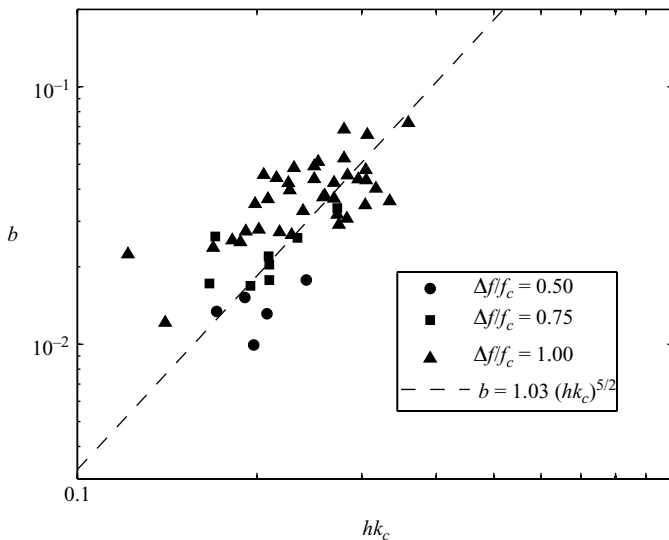
FIGURE 13. Plot of b versus the local slope, hk_c . Data for all three bandwidths for singly breaking plunging waves only are shown. The dashed line is a fit of the data to the curve b = \alpha (hk_c)^{5/2} , where \alpha = 1.03 .
