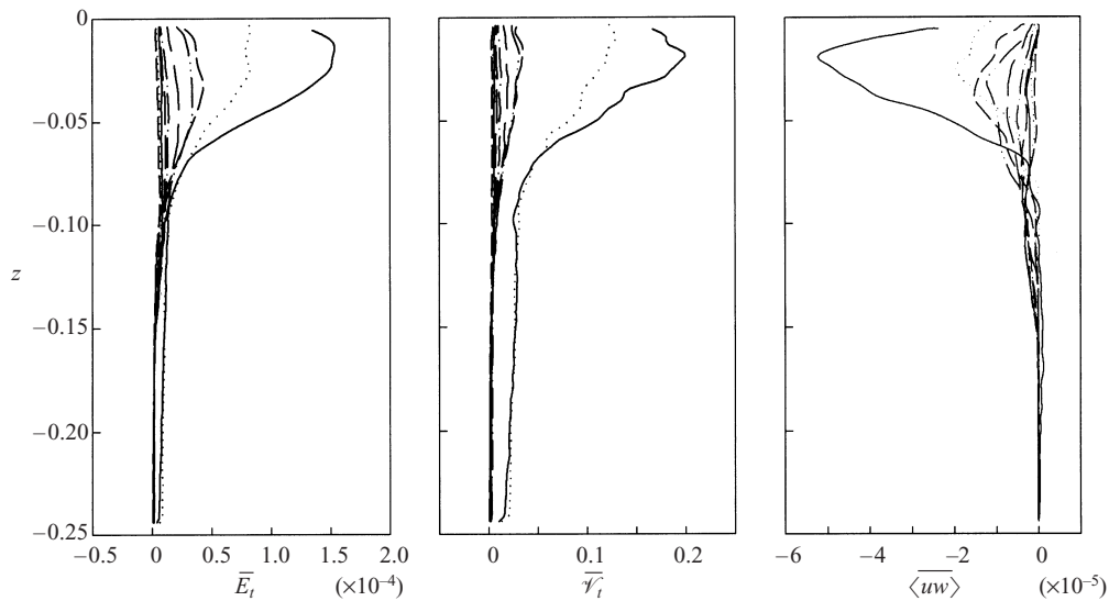
FIGURE 13. Averaged horizontal profiles of the mean turbulent kinetic energy, \bar{E}_t , the mean square turbulent vorticity, \overline{\mathcal{V}_t^2} , and the Reynolds stress, \langle uw \rangle . Note that the horizontal average is over a length of 0.7 defined by the vertical lines in figure 9 which move at the speed of the turbulent cloud.
