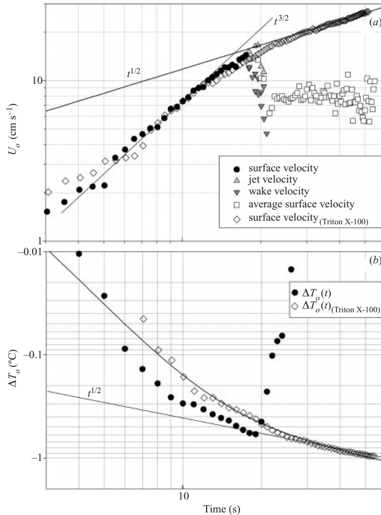
FIGURE 18. (a) Surface velocity for a final wind speed of 5 \text{ m s}^{-1} and a fetch of 10.72 m with and without Triton X-100 added to the water (cf. figure 17a); the solid lines are the linear stress ( t^{3/2} -dependence) and the constant stress ( t^{1/2} -dependence) relations. (b) The data of figure 17(b) and the prediction from equation (3.18) where the surface heat flux Q(t) is based on the wind speed according to equation (3.19). Also shown is the constant heat flux ( t^{1/2} -dependence).
