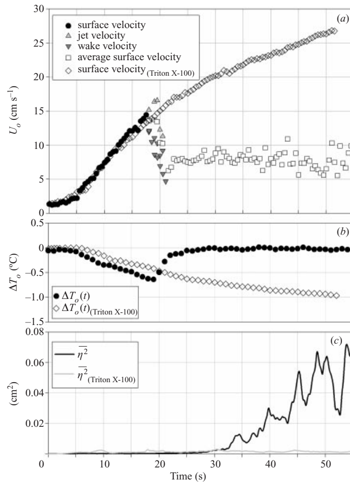
FIGURE 17. (a) Surface velocity, (b) surface temperature deviation for a final wind speed of 5 \text{ m s}^{-1} and a fetch of 10.72 \text{ m} with and without Triton X-100 added to the water (the data of figures 10 and 13 are plotted in (a) and (b) respectively). (c) Shows the time series of the variance of the surface wave height with and without added surfactant.
