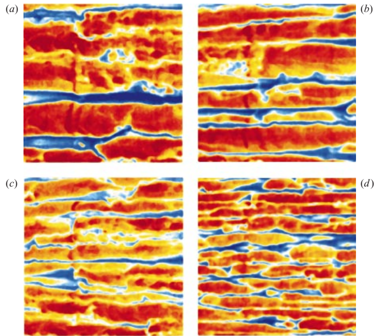
FIGURE 5. Surface temperature fields for final wind speeds of (a) 3, (b) 4, (c) 5, and (d) 6 \text{m s}^{-1} at a fetch of 10.72 m and at similar stages in the evolution of the flow. Times shown are 43.8, 28.3, 21.3 and 14.3 s, respectively.
