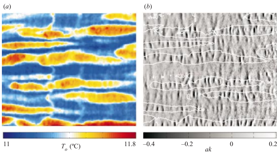
FIGURE 15. (a) Surface temperature (from figure 4c), and (b) along-wind slope at the same location at time t = 19.8 s. Note the correlation between the warm upwelling regions and the regions of larger wave slope. Wind and waves are travelling left to right. The image size is 36.8 \text{ cm} \times 27 \text{ cm} .
